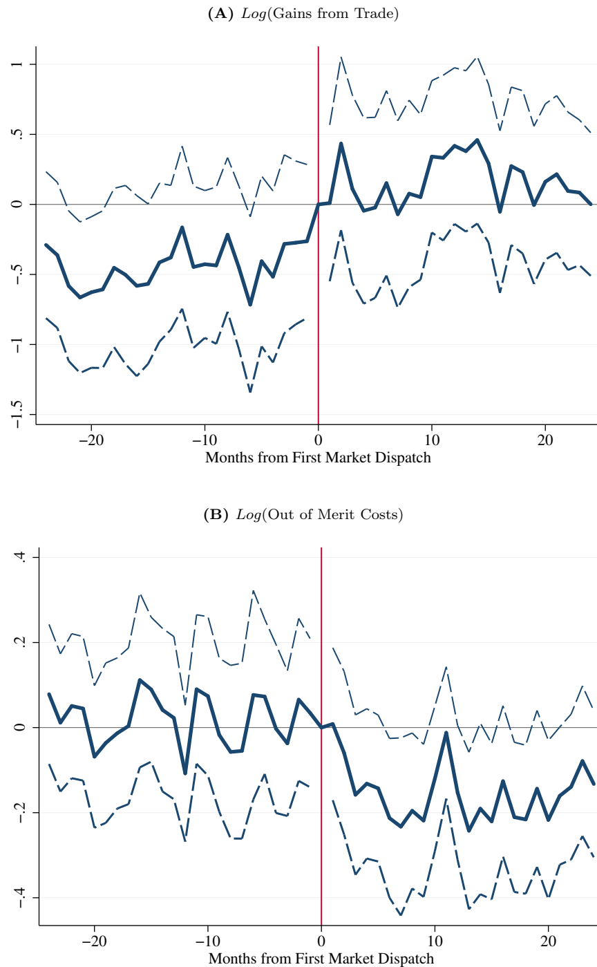
Figure B.8: Main Allocative Efficiency Results: No Spot Market Price Estimation
