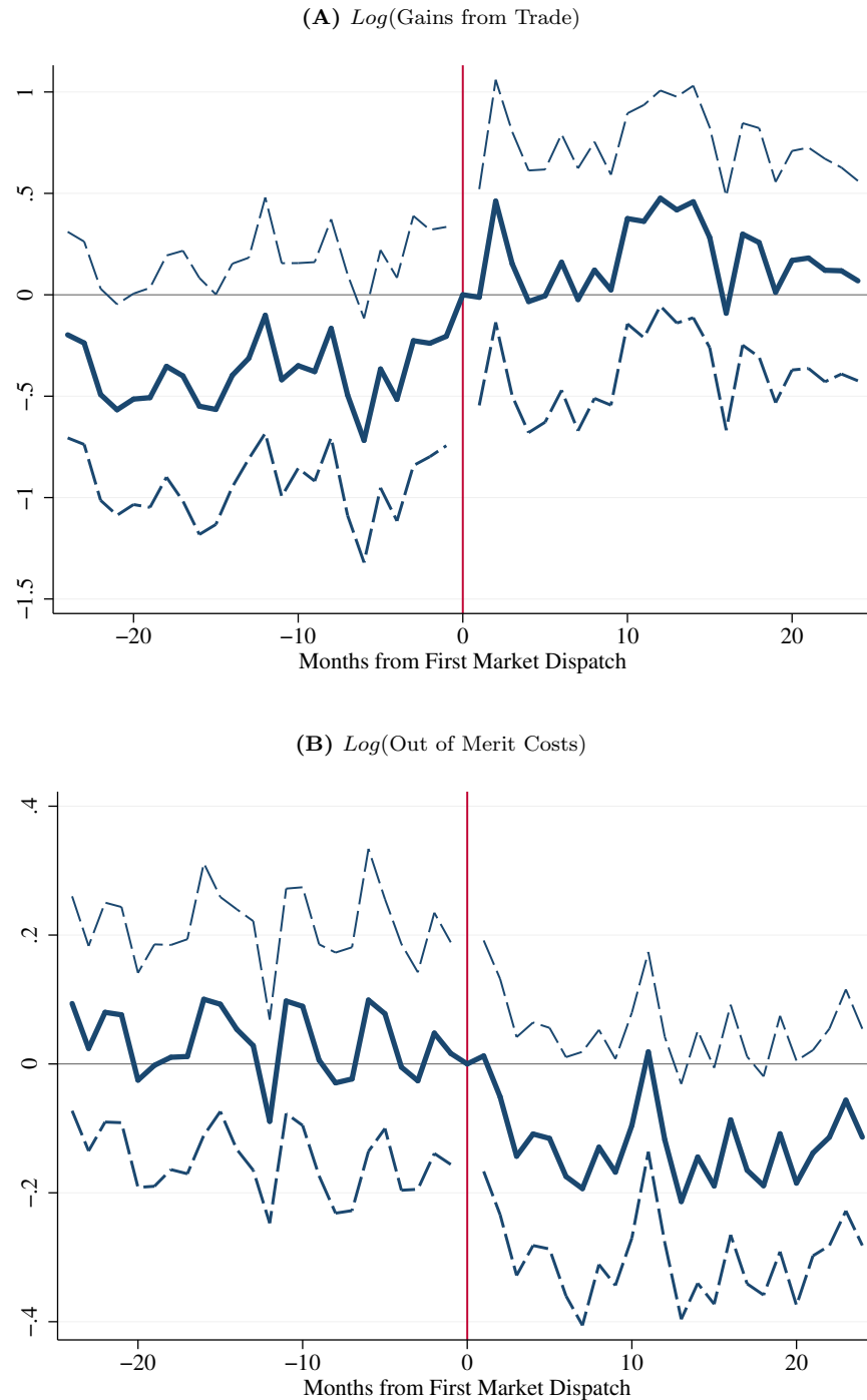
Figure B.7: Main Allocative Efficiency Results: Publicly-Available Fuel Prices
