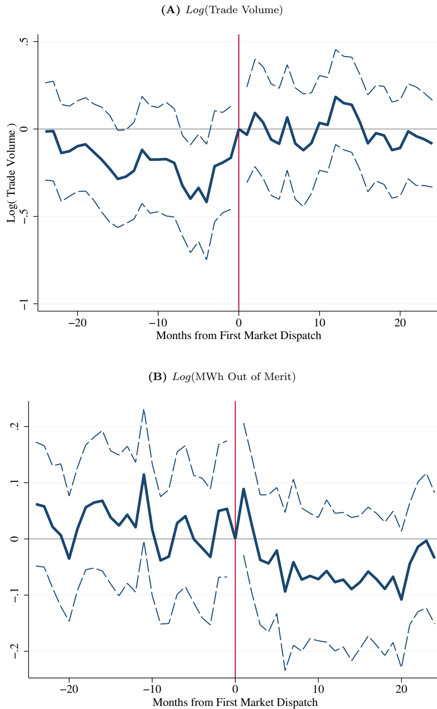
Figure B.4: Main Quantity Results: No Load or Cost Controls
