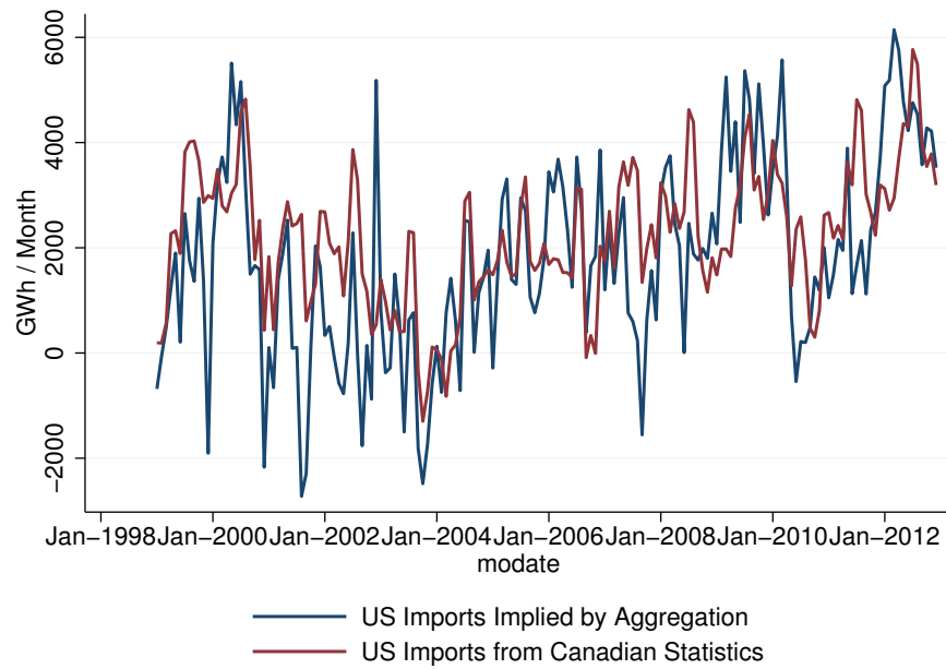
Figure A.2: Monthly Net Imports from Canadian Statistics versus Load-Generation Mismatch
