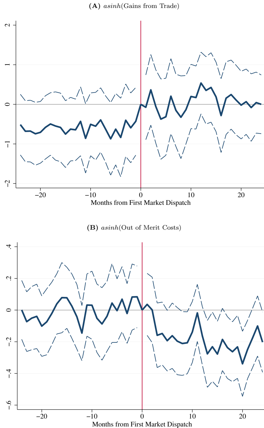
Figure B.6: Main Allocative Efficiency Results: Inverse Hyperbolic Sine Transformation
