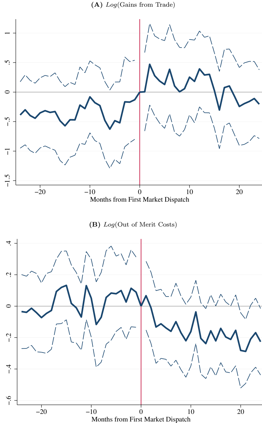
Figure B.5: Main Allocative Efficiency Results: No Load or Cost Controls
