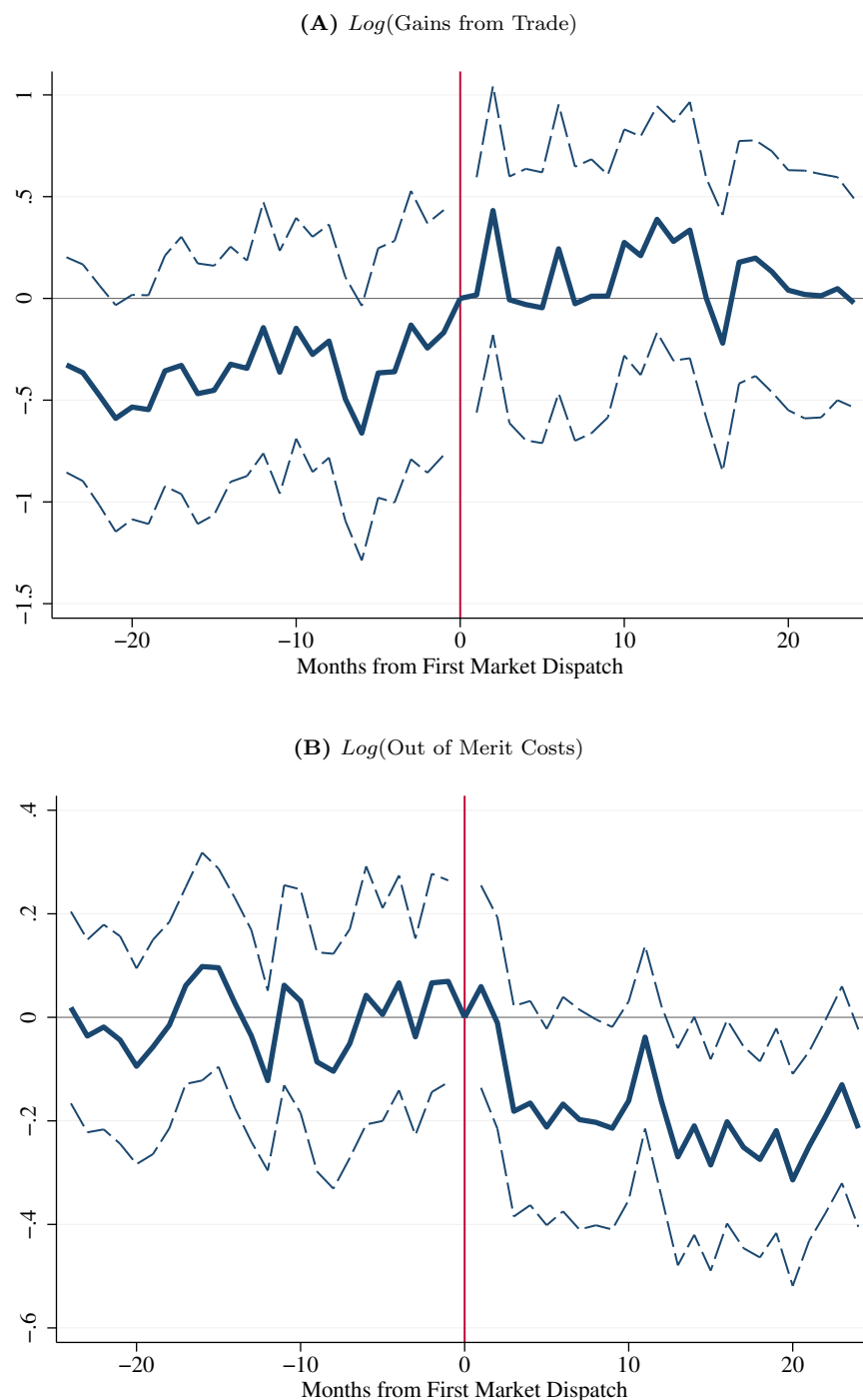
Figure B.9: Main Allocative Efficiency Results: Zero Cost Reservoir Hydropower
